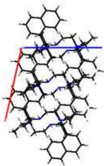
Figure 3. Packing diagram, viewing along the b axis of the unit cell
