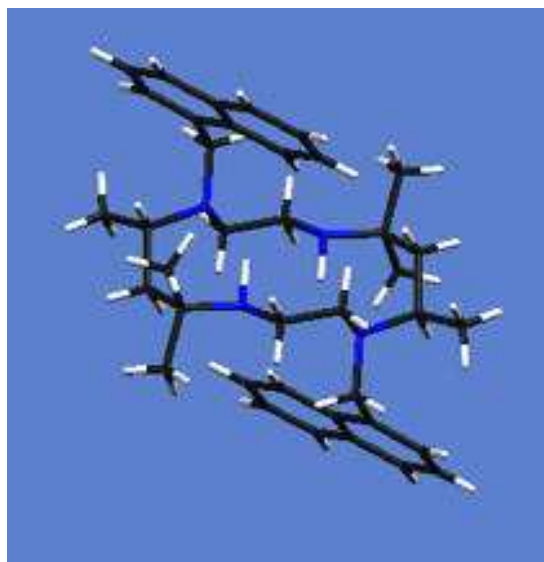
Figure 2. Mercury 1.1 display of meso-5,5,7,12,12,14-hexamethyl-1,4,8,11-tetraazacyclotetradecane-1,8-di-(1-methylnaphthalene)
