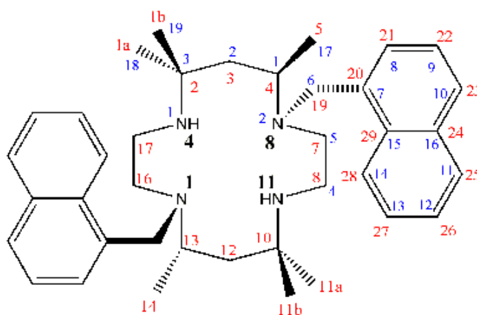
Figure 1. Structural representation of the 1,8-di-(1-methylnaphthalene) derivative of tet A
